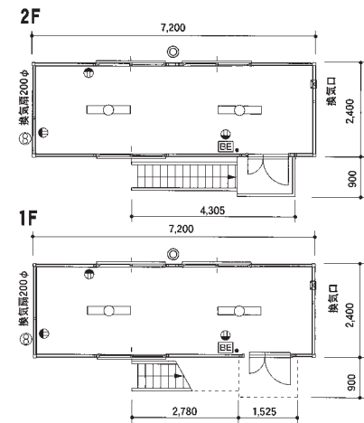
SH-H6 2階建
