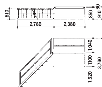
SH-HP型／階段
